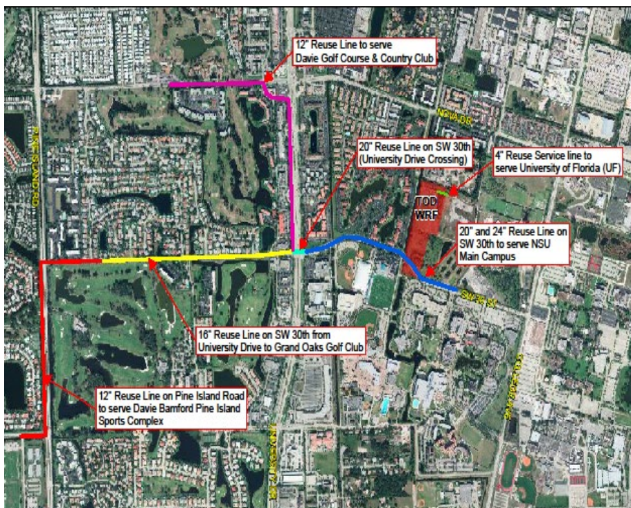
Map. Town of Davie Utilities Water Reclamation Facility (WRF) – Reclaimed Water availability layout
