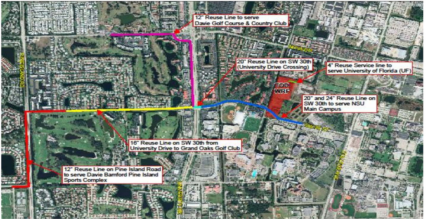
Map. Town of Davie Utilities Water Reclamation Facility (WRF) – Reclaimed Water availability layout
