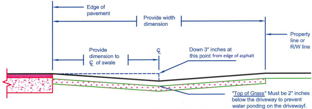
SWALE WITHOUT SIDEWALK
