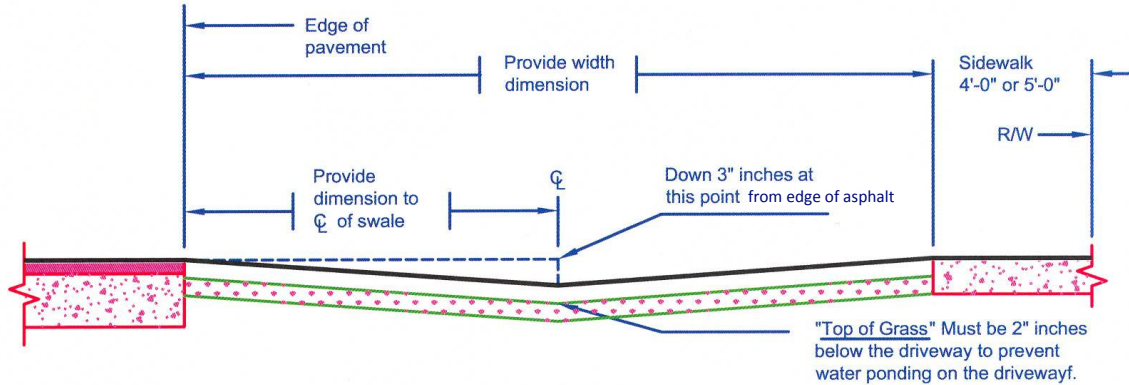
SWALE WITH SIDEWALK
