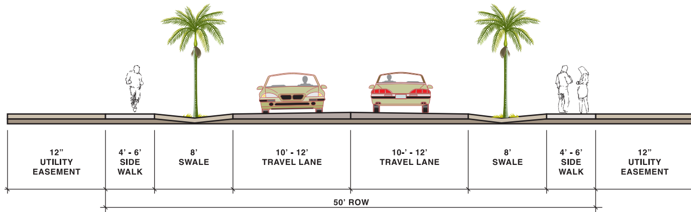
LOCAL URBAN 50' RIGHT-OF-WAY
