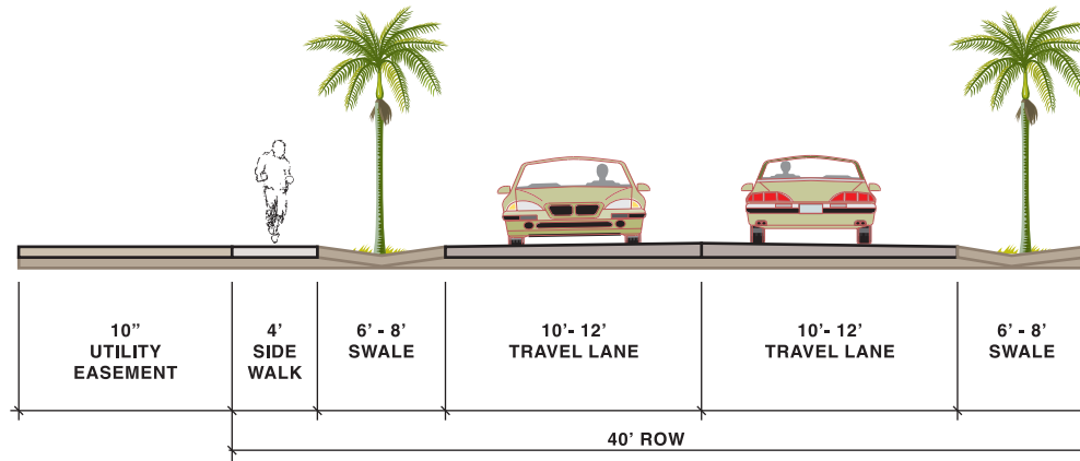
LOCAL RURAL 40' RIGHT-OF-WAY
